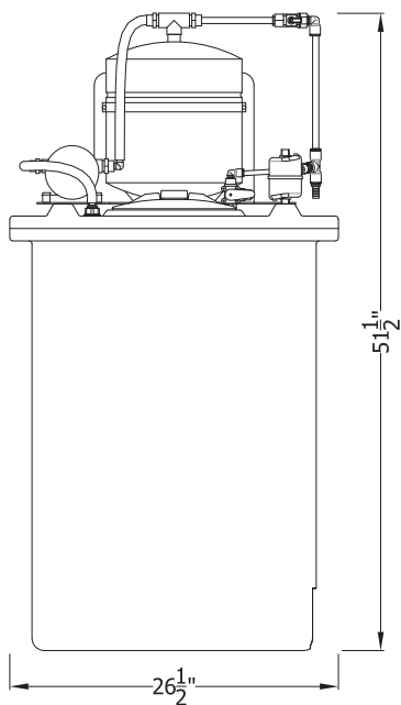
Storage Tank Assembly - 120V
