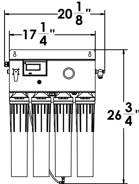
Water Processor - 120 VAC / 6 Watts
