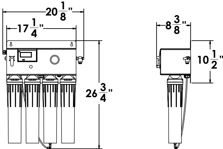
Water Processor Assembly - 120V
