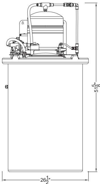
Storage Tank Assembly - 120V
