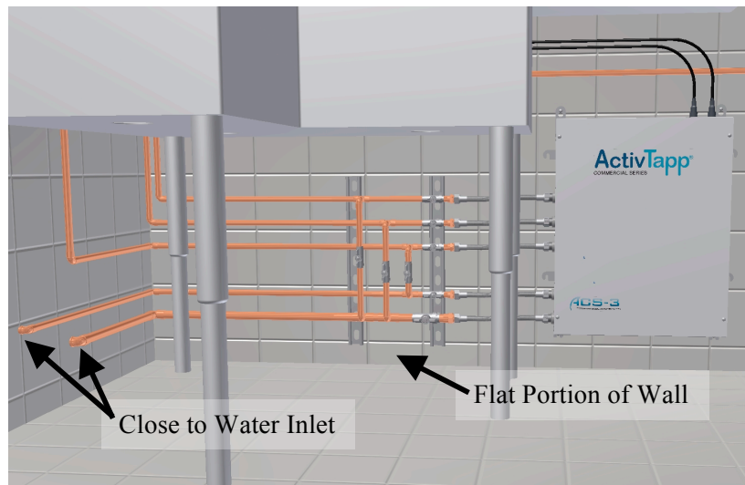
Figure 2 – Mounting Location
