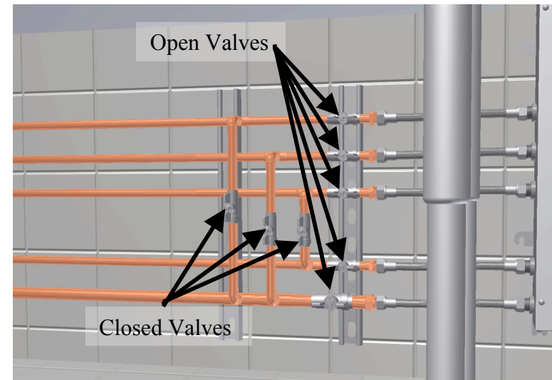
Figure 8 – Manifold Valve Settings
