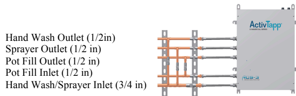
Figure 4 – ACS-2 Inlet and Outlet
